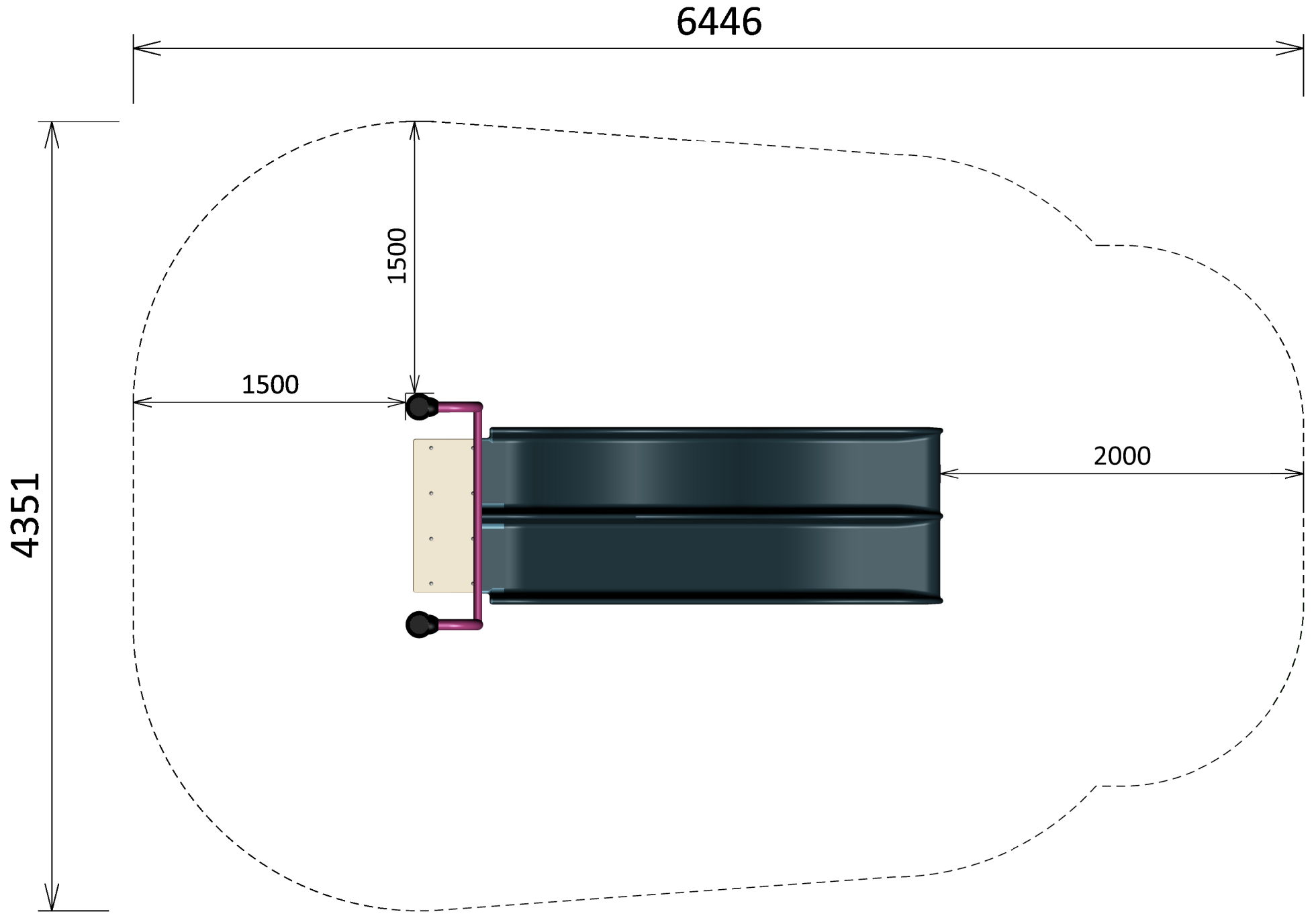
EMBANKMENT SLIDE 1200 DOUBLE WITH RAIL
