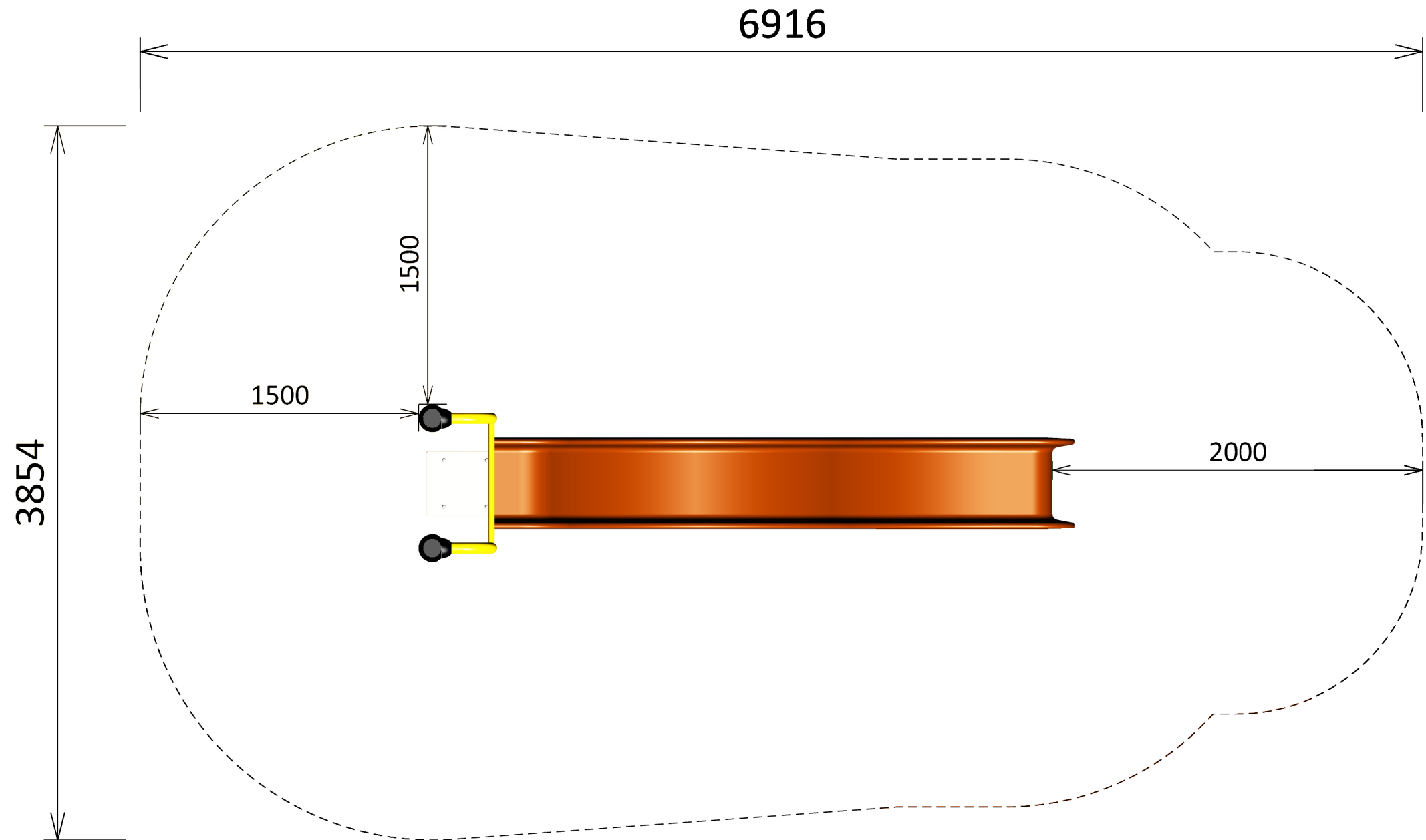
EMBANKMENT SLIDE 1600 WITH RAIL
