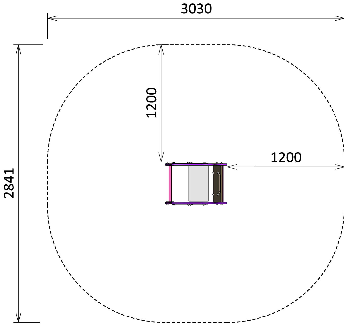
ACCESSIBLE SCUTTLE ROCKER (SE-70)
